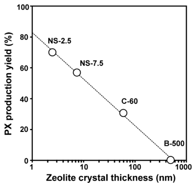
Figure 4. Plot for zeolite crystal thickness versus PX production yield of NS-2.5, NS-7.5, C-60 and B-500 catalysts. Reaction conditions: 0.2 g of catalyst, 25 ml of 2,5-dimethylfuran, 50 bar of ethylene, 75 ml of n -heptane (solvent), 523 K, 24 h.
