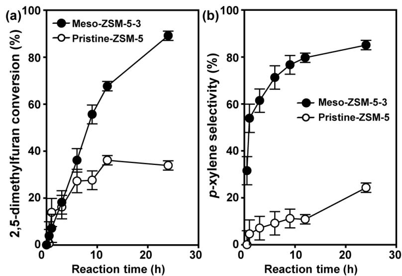
Figure 7. Conversion of 2,5-dimethylfuran (a) and p -xylene selectivity (b) over pristine and desilicated MFI zeolite catalysts as a function of reaction time. Reaction conditions: 0.2 g of catalyst, 25 ml of 2,5-dimethylfuran, 50 bar of ethylene, 75 ml of n -heptane (solvent), 523 K.
