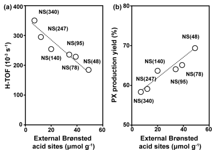
Figure 5. Plot for External Brønsted acid sites versus H-TOF (a) and PX production yield (b) of NS-2.5-( x ) ( x = 48, 78, 95, 140, 247 and 340 ). Reaction conditions: 0.2 g of catalyst, 25 ml of 2,5-dimethylfuran, 50 bar of ethylene, 75 ml of n -heptane (solvent), 523 K, 24 h.
