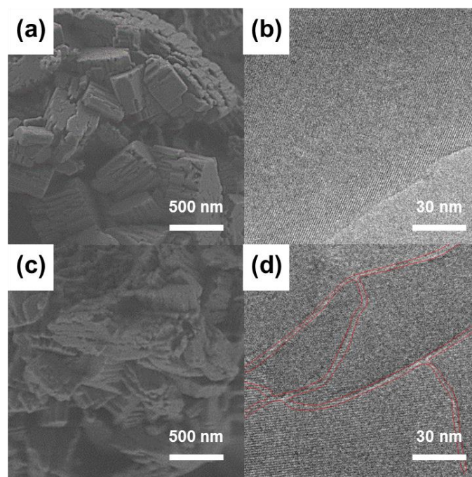
Figure 6. Representative SEM and TEM images of pristine commercial ZSM-5 ((a), (b)) and Meso-ZSM-5-3 sample ((c), (d)).
