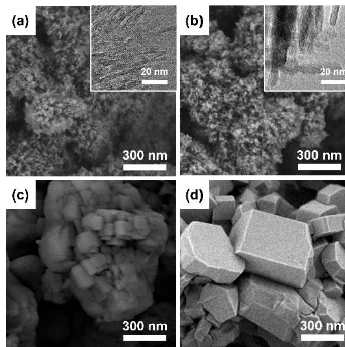
Figure 1. Representative SEM and TEM images of (a) NS-2.5, (b) NS-7.5, (c) C-60 and (d) B-500.
