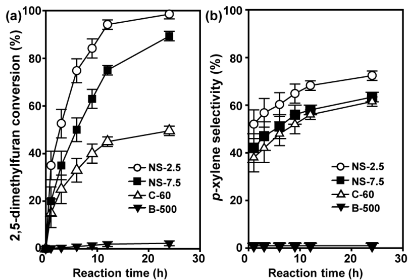
Figure 3. Conversion of 2,5-dimethylfuran (a) and p -xylene selectivity (b) over NS-2.5, NS-7.5, C-60 and B-500 as a function of reaction time. Reaction conditions: 0.2 g of catalyst, 25 ml of 2,5-dimethylfuran, 50 bar of ethylene, 75 ml of n -heptane (solvent), 523 K.
