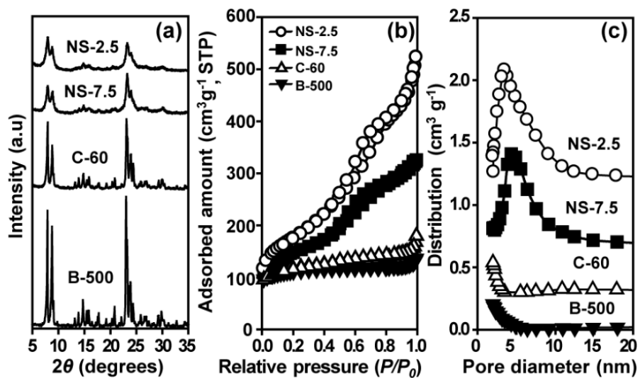
Figure 2. Powder XRD patterns (a), nitrogen sorption isotherms (b), and pore size distribution corresponding to the adsorption branch (c) of NS-2.5, NS-7.5, C-60, and B-500.
