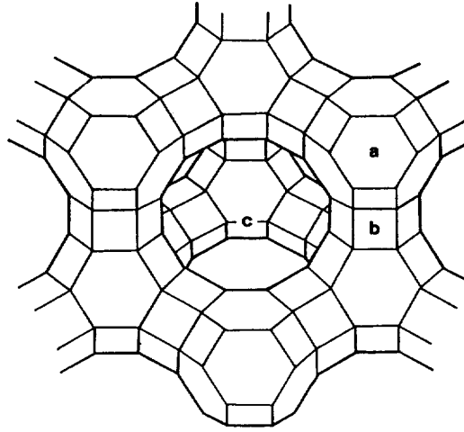
Fig. 1. The framework of faujasite-type zeolite containing (a) sodalite cage, (b) hexagonal prism and (c) supercage. Vertices represent oxygen bridges between silica and alumina tetrahedra. The silica and aluminum atoms are located at the intersections of these vertices.
