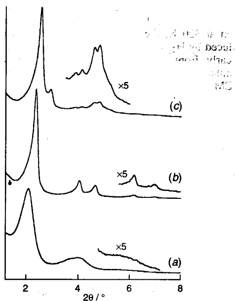
Fig. 2 X-Ray diffraction patterns of mesoporous molecular sieves KIT-1 (a), MCM-41 (b) and MCM-48 (c) after calcination in an \text{O}_2 flow at 813 K
