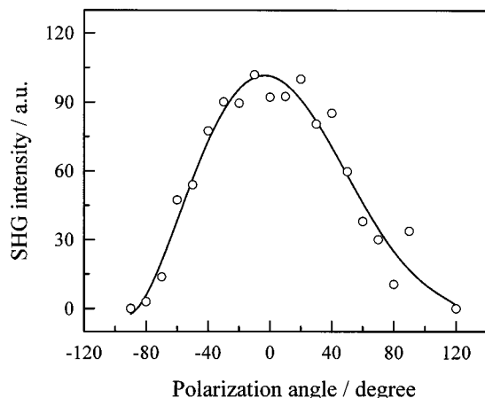
Figure 5. Second harmonic generation effects of the ordered mesoporous silica plate after the adsorption of p -nitroaniline, plotted against the polarization angle with respect to the channel direction.
