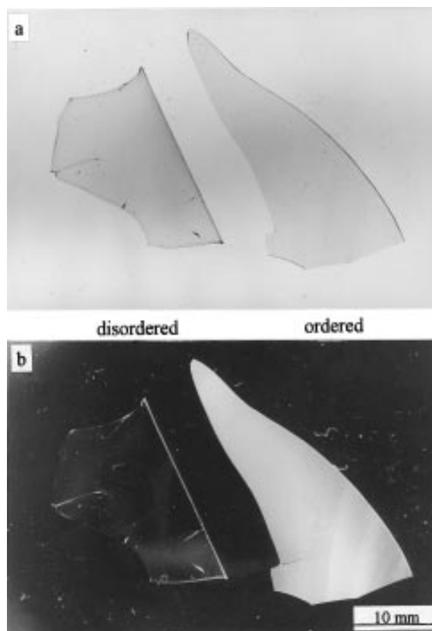
Figure 4. Photographs of calcined mesoporous silica plates with ordered and disordered channel structures placed between two Polaroid plates: (a) with polarization of the Polaroid plates oriented to the same direction and (b) perpendicular.
