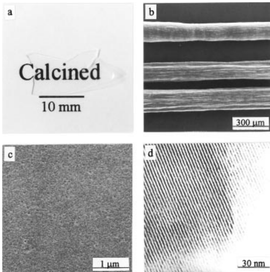
Figure 1. Photograph (a), scanning electron micrographs (b, c), and transmission electron micrograph (d) for ordered mesoporous silica after calcination at 823 K. The scanning electron micrographs were recorded on a Philips 535M apparatus operating at 20 kV. The transmission electron micrograph was obtained with JEM 200EX (JEOL) apparatus operating at 100 kV from thin edges of microparticles, which were obtained by grinding the sample shown in (a) using an agate mortar.
