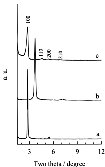
Figure 2. X-ray diffraction patterns for ordered mesoporous silica samples: (a) single free-standing plate (0.5 mm thick) as synthesized, (b) after calcination of the plate, and (c) after grinding the as-synthesized plate in an agate mortar. The patterns were obtained from a Rigaku D/MAX-III instrument at room temperature using Cu K\alpha radiation. Diffractograms (a) and (b) were obtained with the reflecting plane of X-rays parallel to the flat surface of the plate. XRD patterns for the as-synthesized and calcined thin film coated on slide glass were very similar to the XRD patterns for the free-standing plate.
