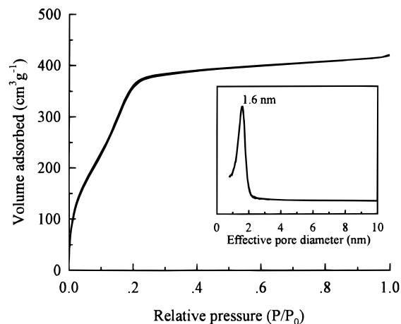
Figure 3. Argon adsorption–desorption isotherms for the ordered mesoporous silica plate after calcination, obtained at liquid argon temperature. The isotherm was obtained on a Micromeritics ASAP 2010 apparatus with volumetric method. Relative pressure is P/P_0 , where P is the equilibrium pressure of the adsorbate at temperature and P_0 is the saturation pressure of the adsorbate at the temperature. Volume adsorbed is at STP. Inset: the corresponding pore size distribution curve obtained by the BJH (Barrett–Joyner–Halenda) analysis.
